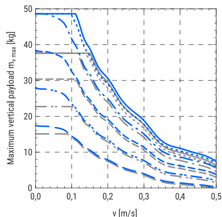
10 × 10 with a stepper motor □56
