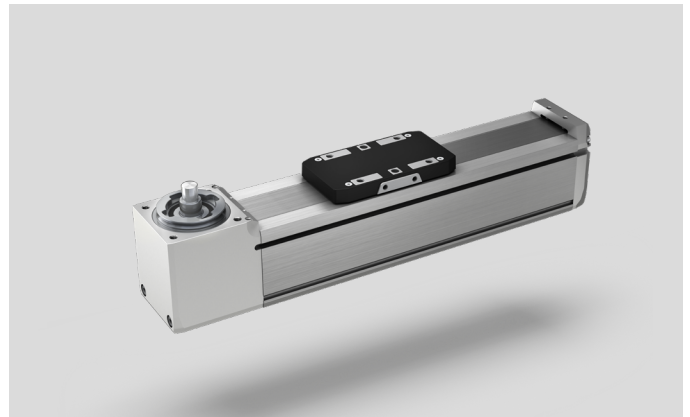
MGTB without a preassembled motor
