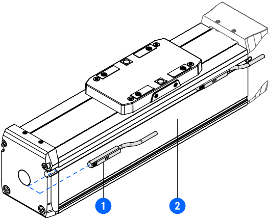
1 – Magnetic field sensor. 2 – Profile of the mini linear unit MGBS or MGTB.
